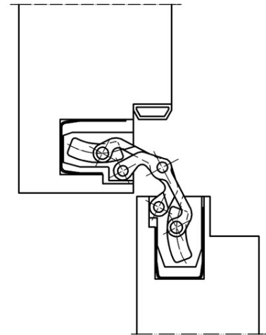
block frame 90°
