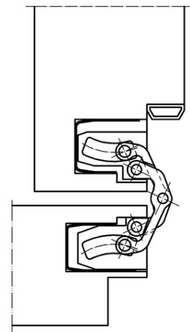
block frame 180°
