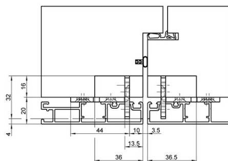
cross section 2
