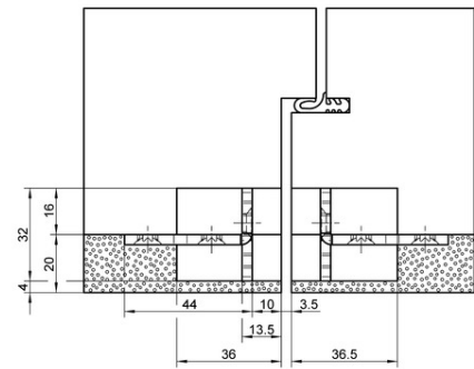
cross section 1
