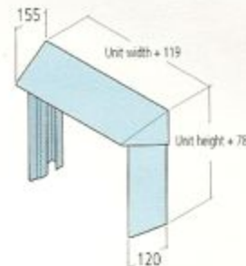
PRISMA® stainless steel casing
