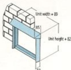
PRISMA® stainless steel plaster frame
