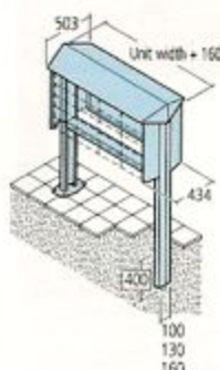
PRISMA® stainless steel casing
