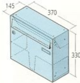
Mail box 370 x 330 x 145 mm
