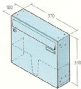
Mail box 370 x 330 x 100 mm
