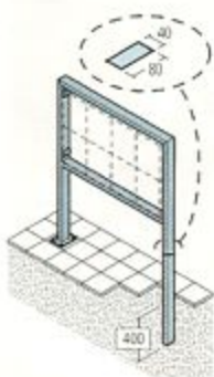
Stainless steel rectangular tube frame
