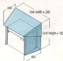
PRISMA® stainless steel casing
