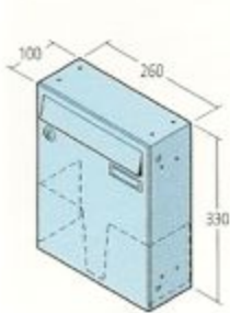
Mail box 260 x 330 x 100 mm
