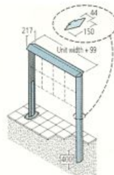
PRISMA® stainless steel casing for 100 mm deep boxes
