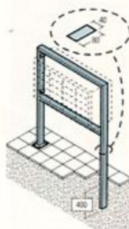
Stainless steel rectangular tube frame
