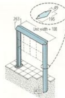
PRISMA® stainless steel casing for 145 mm deep boxes
