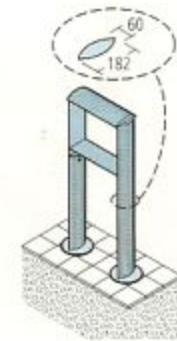
CONVEX® stainless steel casing available on request
