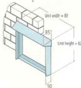
PRISMA® stainless steel plaster frame
